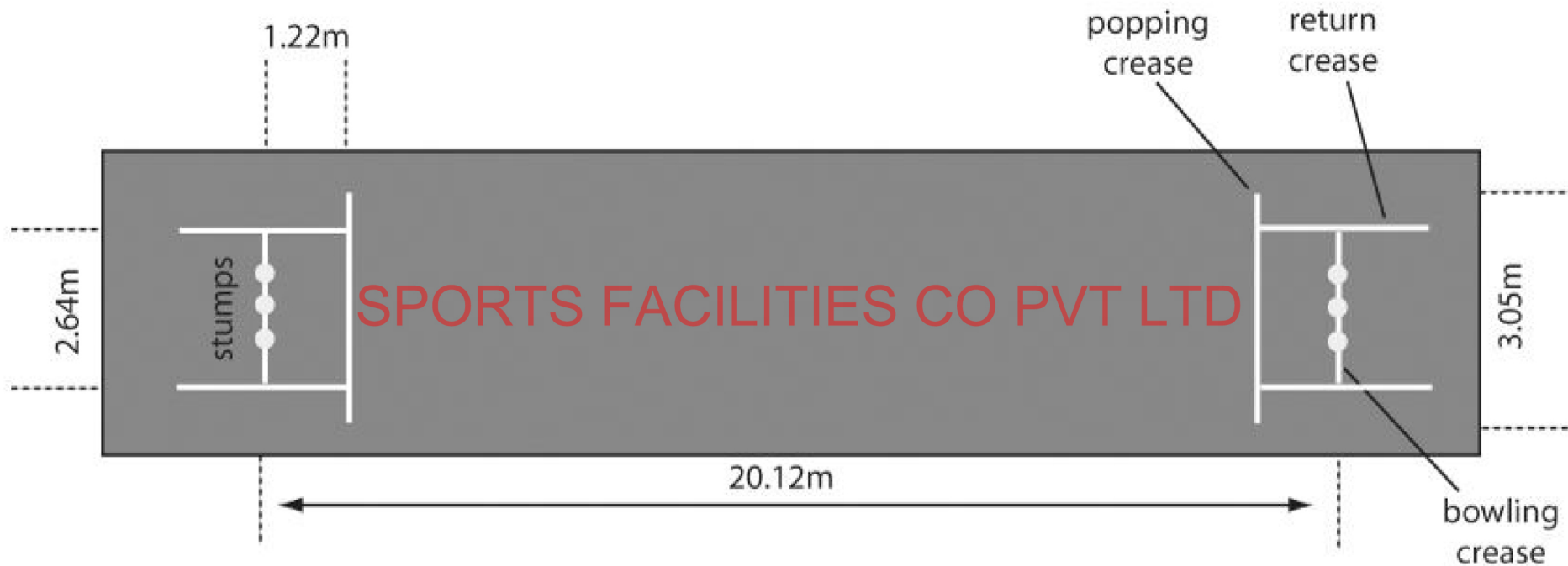
LAYOUT OF CRICKET PITCH
