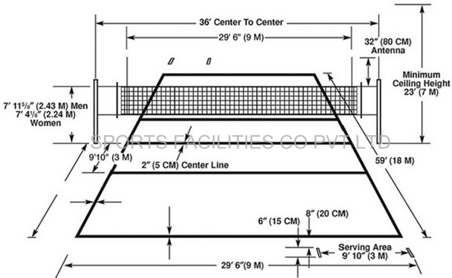
LAYOUT OF THE VOLLEYBALL COURT
